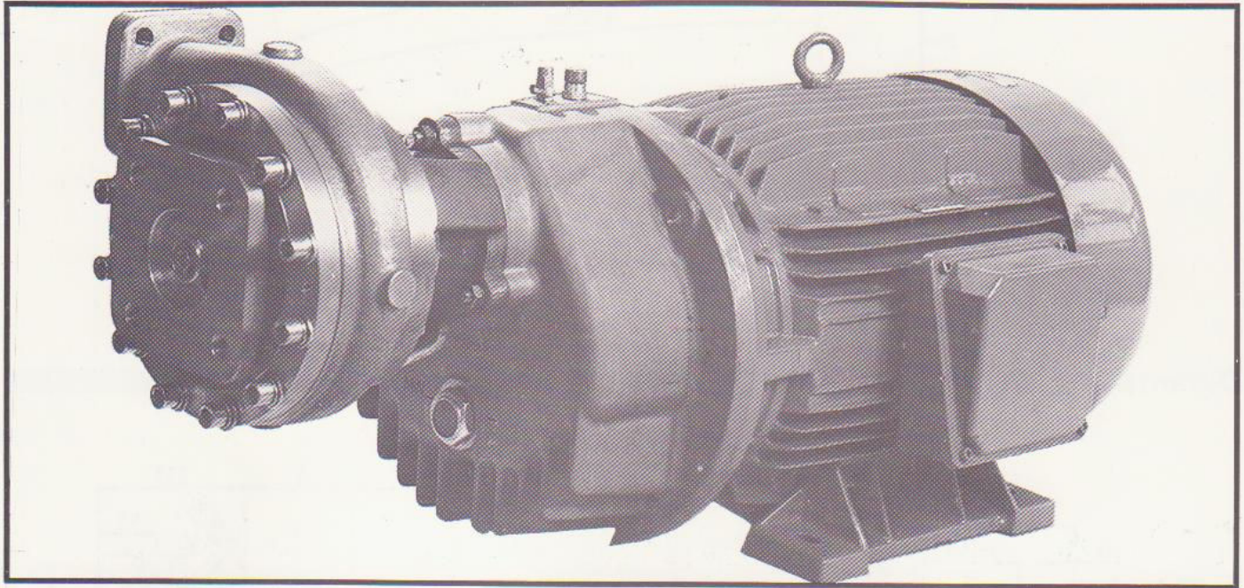
Standard road-tanker pump with 22 or 30 kw electric motor
