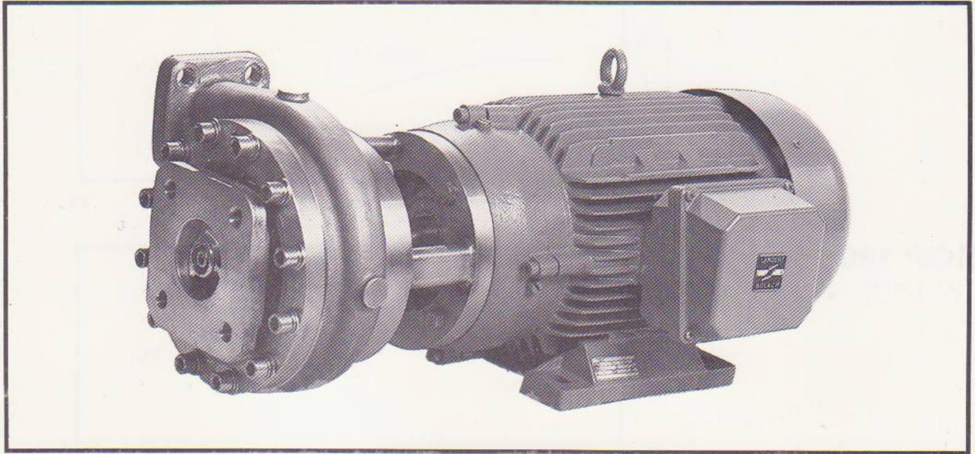
DCP 180-4, 5 for low pressure tank-to-tank transfer with 7.5 kw electric motor
