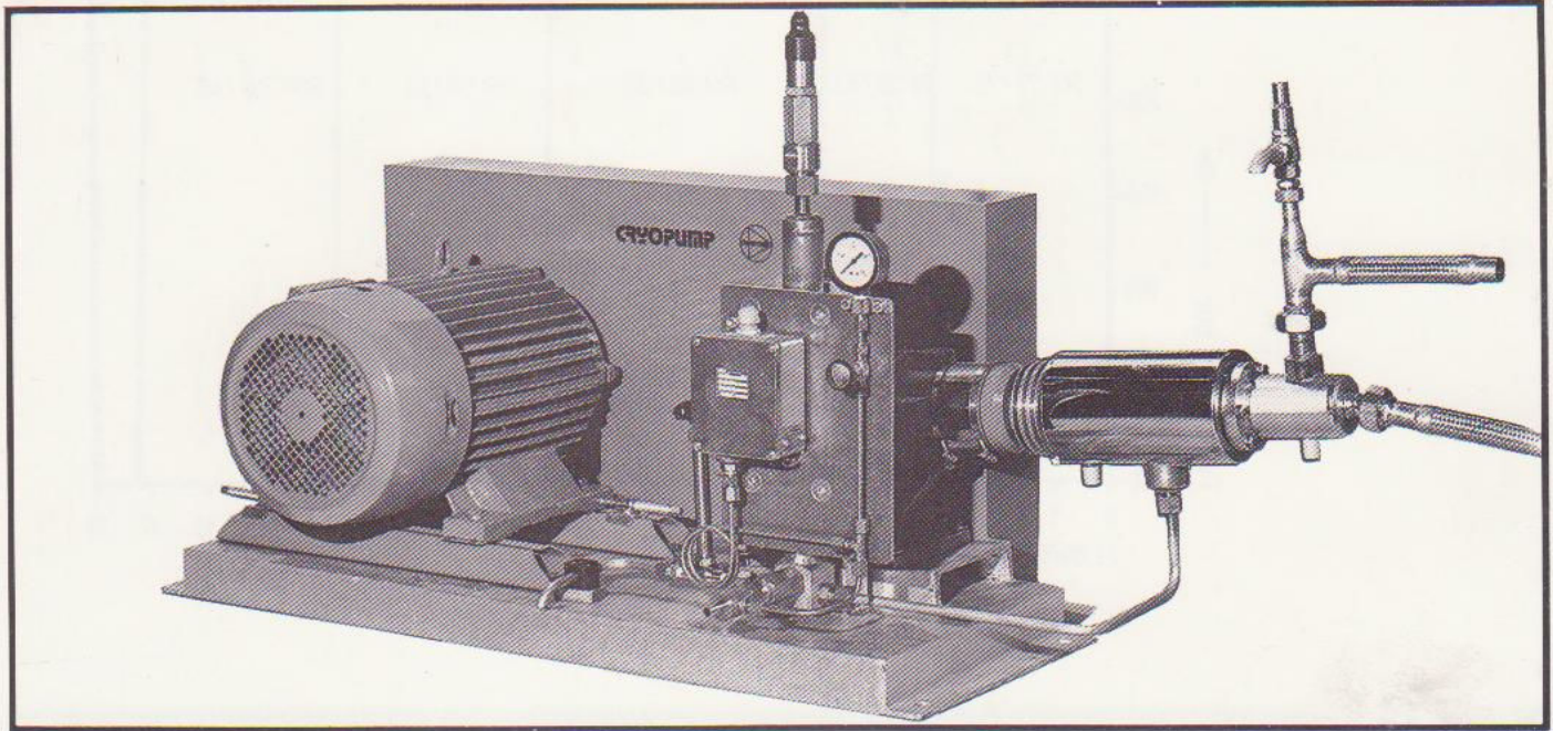
Standard installation for cylinder-filling up to 300 bar pressure
